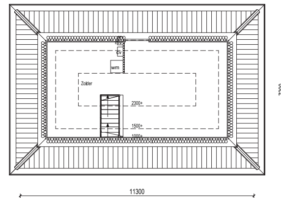
Basis zolder
