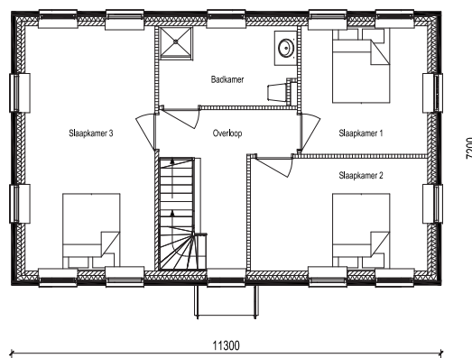
Basis verdieping 1
