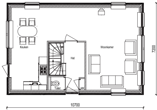
Basis begane grond
